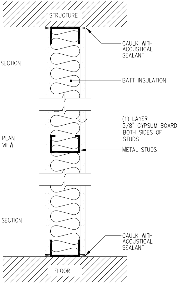
W1 STC 45 - ACOUSTICAL WALL
