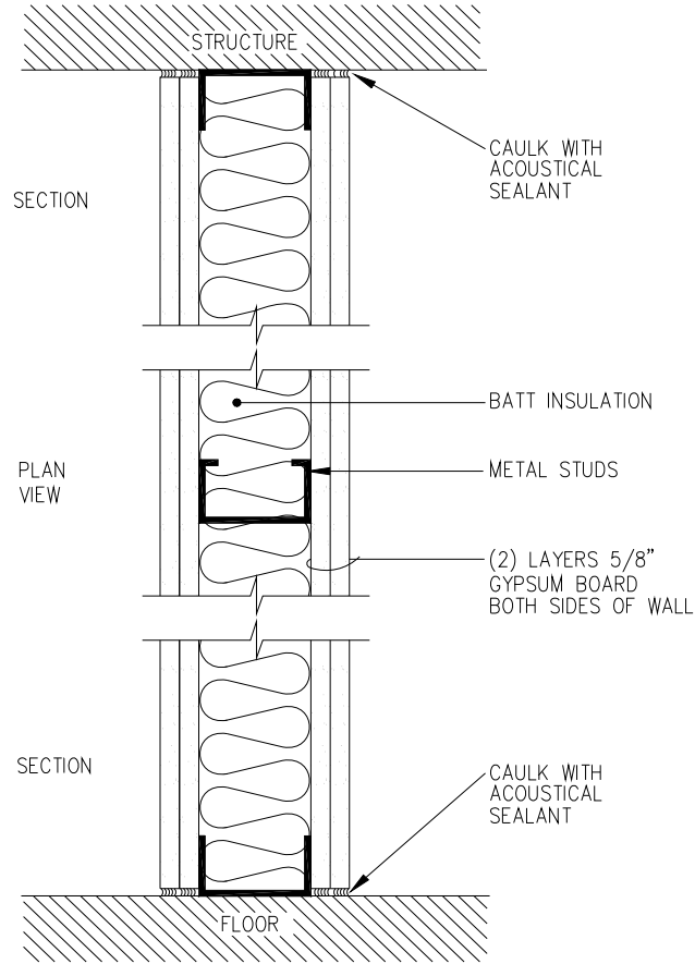
W2 STC 55 - ACOUSTICAL WALL
