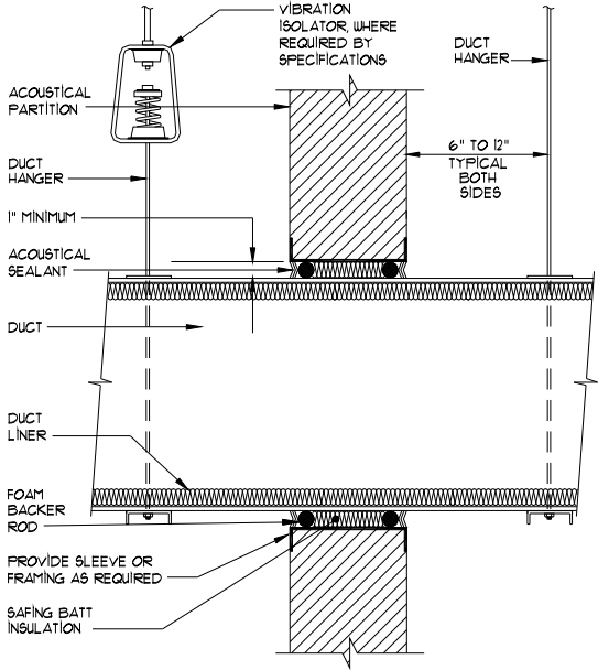
4 TYPICAL DUCT PENETRATION THROUGH ACOUSTICAL PARTITION
